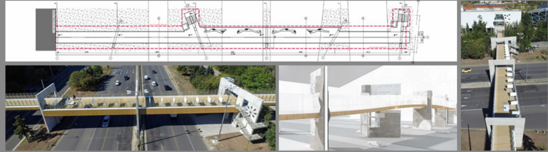
PEDESTRIAN BRIDGE OVER "TSARIGRADSKO SHOSE" BLVD. - SOFIA, BULGARIA
